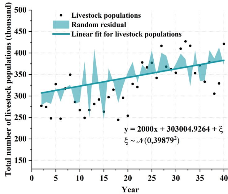
Figure 3. The linear fitting curve of livestock populations.
